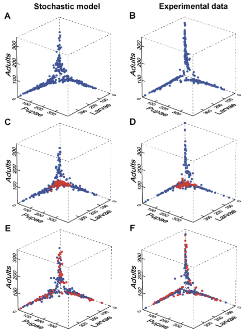
Fig. 3 Phase space plots of numbers of larvae, pupae, and adults for the stochastic model and experimental data. The simulations are from the stochastic LPA model (2) with the same initial conditions, number of replicates, and number of census points as the experimental treatments and the same parameter values as Fig. 1. To de-emphasize the effects of transient changes, excluded from the plots are all simulated and observed data for weeks 0–14 and all simulated and observed data for weeks 134–148 in the in-box and out-box treatments. The blue symbols are for the unperturbed populations; the red symbols are for data collected after the perturbation protocols were started at week 134. (A) Data from three independent realizations of the stochastic LPA model. (B) Data from the three replicate experimental populations in the control treatment group. (C) Data from three independent realizations of the stochastic LPA model using the in-box perturbation protocol. (D) Data from the three replicate experimental populations in the in-box treatment group. (E) Data from three independent realizations of the stochastic LPA model using the out-box perturbation protocol. (F) Data from the three replicate experimental populations in the out-box treatment group.
