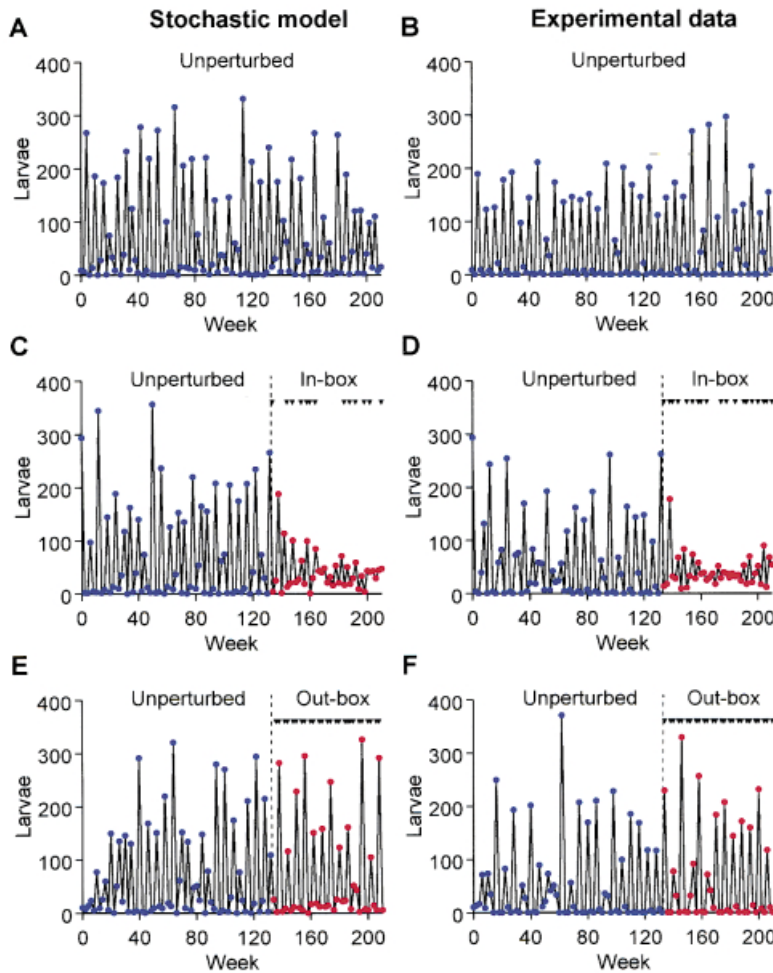
Fig. 2 Time series plots of numbers of larvae for the stochastic model and experimental data. The simulations are from the stochastic LPA model (2) with the experimental initial conditions and the same parameter values as Fig. 1. The blue symbols are for the unperturbed populations; the red symbols are for data collected after the perturbation protocols were started at week 134 (dashed lines). The small inverted triangles indicate when the actual perturbations were applied. (A) A realization of the stochastic LPA model. (B) One of the replicate experimental populations from the control treatment group. (C) A realization of the stochastic LPA model using the in-box perturbation protocol. (D) One of the replicate experimental populations from the in-box treatment group. (E) A realization of the stochastic LPA model using the out-box perturbation protocol. (F) One of the replicate experimental populations from the out-box treatment group.
