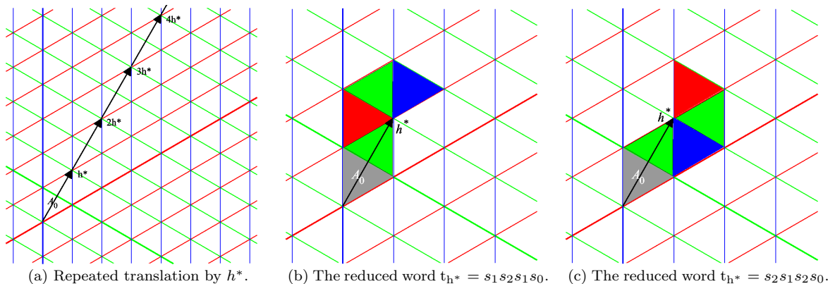
Figure 4: Constructing infinite reduced words in SU(3) .
