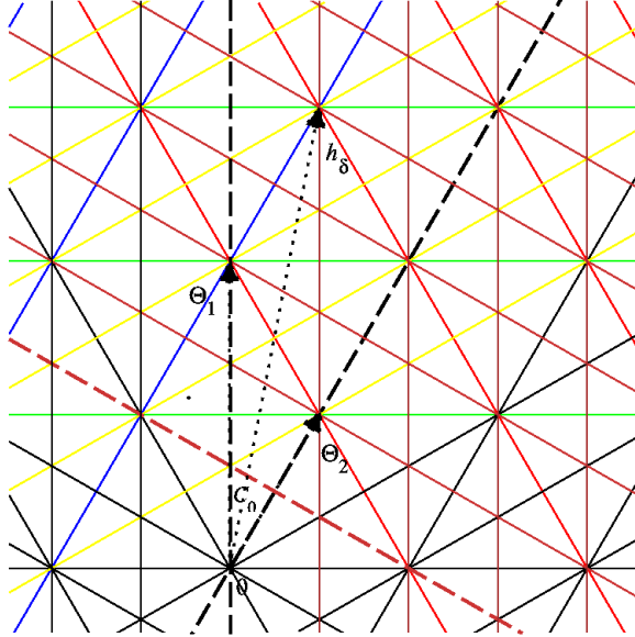
Figure 5: The alcove diagram for G_2 .
