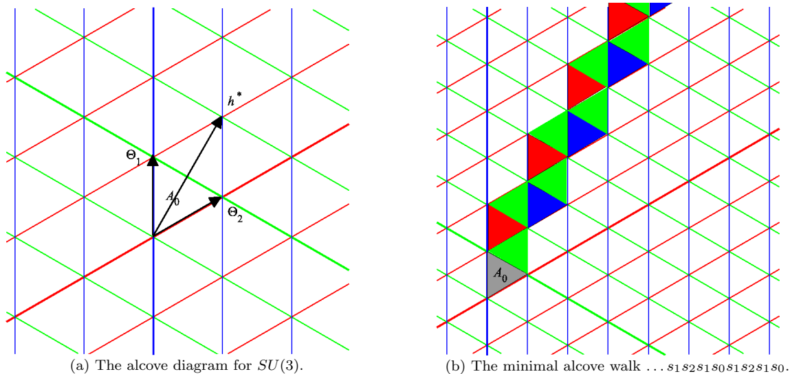
Figure 3: Alcoves for SU(3) .
