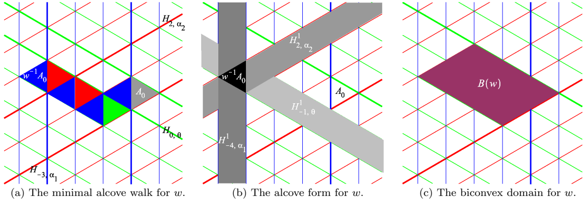
Figure 6: The minimal alcove walk, alcove form, and biconvex domain for w = s_2s_0s_1s_2s_0s_2s_1 .
