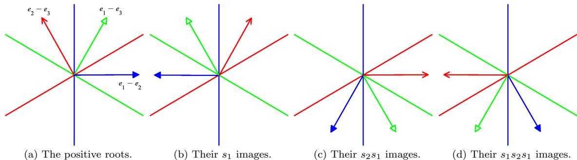
Figure 2: The images of the positive roots (2a) under successive application of s_1 (2b), s_2 (2c), and s_1 (2d).
