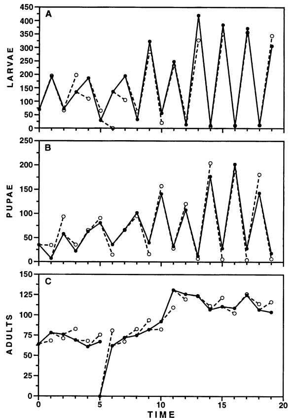
FIG. 17. Time series data (●) and one-step forecasts (○) for replicate B of Desharnais and Liu (1987) where all adults were removed at t = 5 . Solid lines connect the observed census data. The one-step forecasts (dashed-line projections) are based on the parameter estimates obtained from the control cultures.
