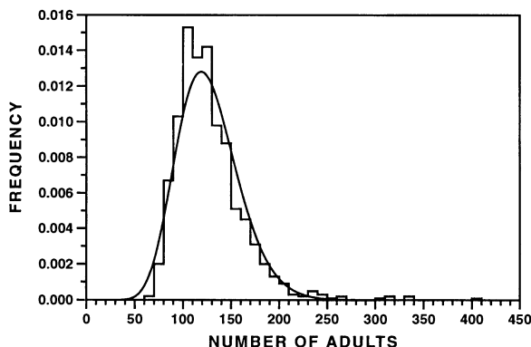
FIG. 22. Histogram of adult numbers for the stochastic LPA model simulated for 1000 time steps using the parameter values (Table 1) and variance-covariance matrix estimated from the control cultures. The smooth curve represents a gamma probability density function fitted to the stochastic realizations.
