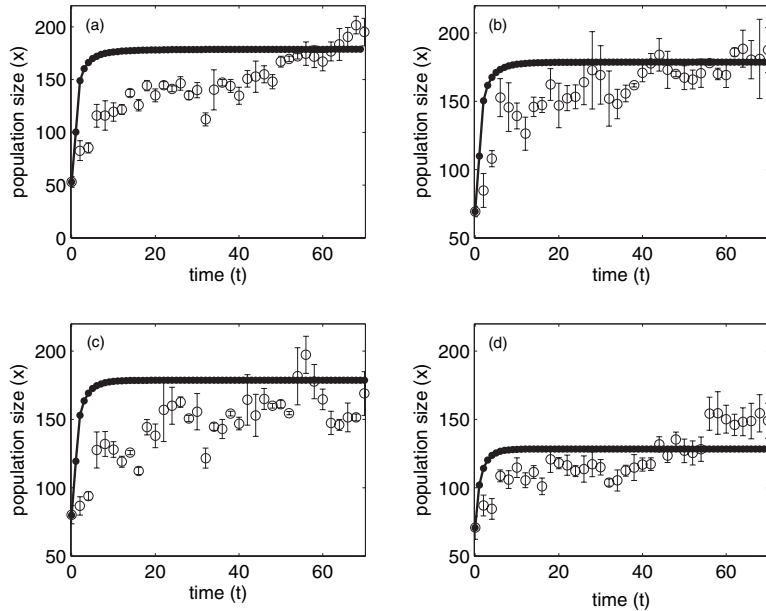
Figure 2: Model results (filled circles) versus experimental data (open circles) with mean standard errors for population dynamics. Treatment 1 (a), treatment 2 (b), treatment 3 (c), control (d). Time represents weeks after the introduction of the + allele, except in the control.
