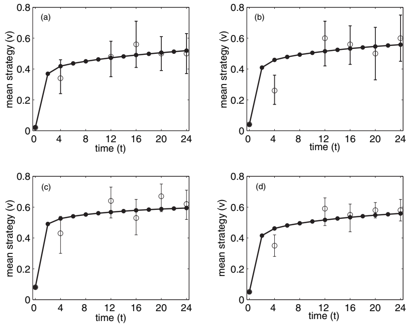
Figure 3: Model results (filled circles) versus experimental data (open circles) with 95% binomial confidence intervals for strategy dynamics. Treatment 1 (a), treatment 2 (b), treatment 3 (c), and mean over these three treatments (d). Time represents weeks after introduction of the + allele. Data in this figure correspond to the first 24 weeks of population data in Figure 2.
