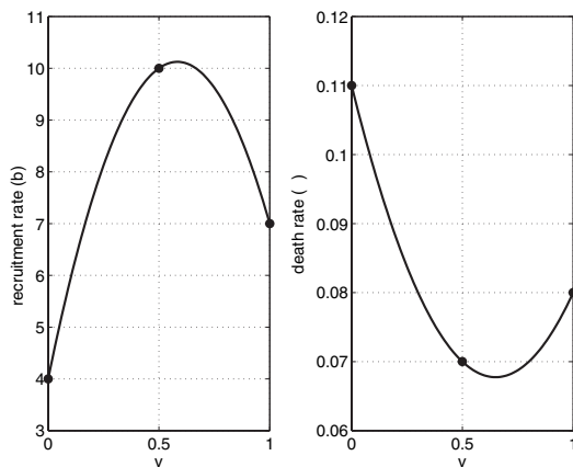
Figure 1: Recruitment ( b ) and death ( \mu ) rates as functions of strategy ( v ).
