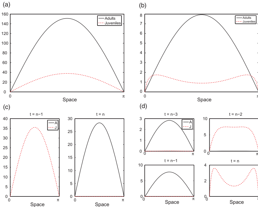
Figure 1. Representative attractors of juvenile–adult IDE model (7). b = 25 \mu_L = \mu_A = 0.2 for all simulations. (a) Temporal equilibrium: D_J = D_A = 0 . (b) Temporal equilibrium, spatial segregation of juveniles and adults: D_J = 0.5 , D_A = 0 . (c) Two-cycle, temporal segregation of juveniles and adults: D_J = 0 , D_A = 0.5 . (d) Four-cycle, temporal segregation of juveniles and adults: D_J = D_A = 0.5 .
