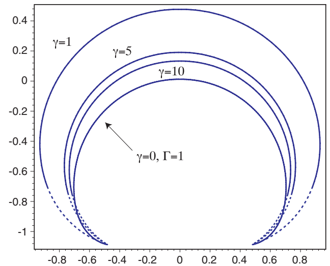
Fig. 10. Appressorial shapes with \Gamma = 10 , \alpha = 3 , \eta = 0.25 with varying nonlinearity \gamma = 1, 5, 10 . The innermost curve corresponds to the shell shape computed with the neo-Hookean free energy with \Gamma = 1 .
