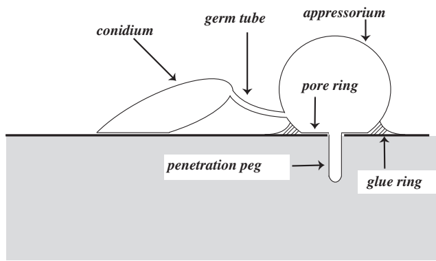
Fig. 1. Pictorial representation of the development of the rice blast fungus.
