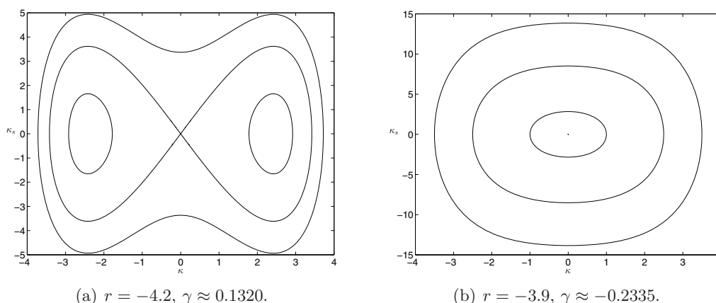
Figure 3. Typical phase plane diagrams associated with system (3.29) for \epsilon = 0.2 , \nu = 4.7 . (a) Curves for \gamma > 0 . The center curve is a homoclinic orbit, and the remaining two curves are periodic orbits of large and small amplitude. (b) Curves for \gamma < 0 . The origin is a center, and all other trajectories are periodic orbits.
