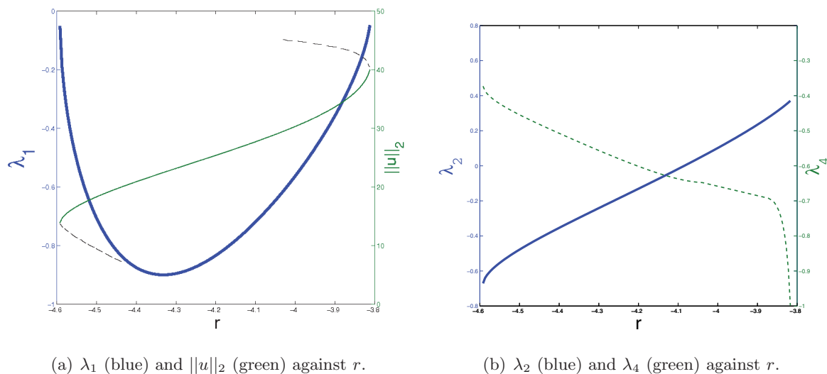
Figure 2. (a) The bifurcation curve of one-dimensional localized solutions ( N(u) = \nu u^2 - u^3 , \nu = 4.7 ) is represented as the L_2 norm squared as a function of the parameter r (thin curves). The dashed part represents the continuation of the solution branch past the saddle nodes at r \approx -4.6, -3.8 . The principle eigenvalue of the stable branch is also shown (thick/blue curve). (b) The expansion coefficients \lambda_2 (solid) and \lambda_4 (dashed).
