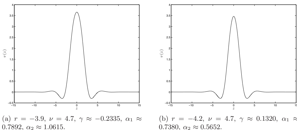
Figure 6. Two one-dimensional cross-sectional solutions of (3.30) used to generate a spatially localized two-dimensional solution. Each profile results in a value of \gamma of differing sign, and consequently each will result in different qualitative behavior arising from (3.20).
