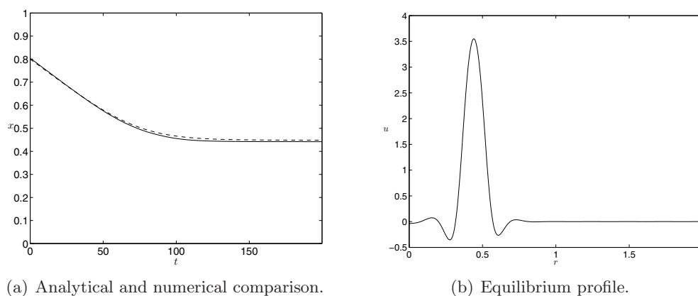
Figure 11. Simulation of (4.5) with parameter values r = -4.088 , R = 2 , \nu = 4.7 , and \epsilon = 0.05 initialized with a single spike centered at \rho = 0.8 . (a) A comparison of the numerical spike location (solid) with the analytical prediction (dashed) of (4.6). (b) The solution profile at equilibrium.
