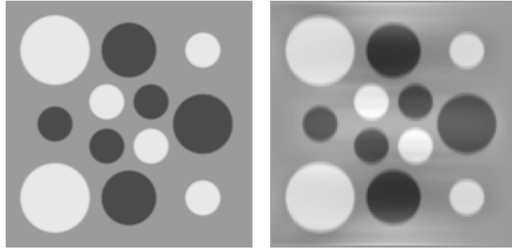
FIGURE 1. Phantom (left) and its EIT reconstruction (right) using focused US modulation.
