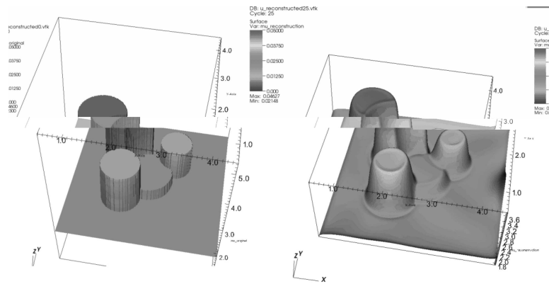
FIGURE 2. Phantom (left) and its OT reconstruction (right) using focused US modulation.
