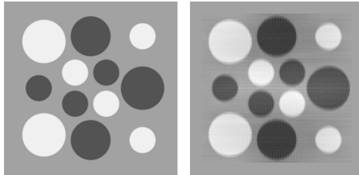
FIGURE 3. AET reconstruction using spherical monochromatic acoustic waves.
